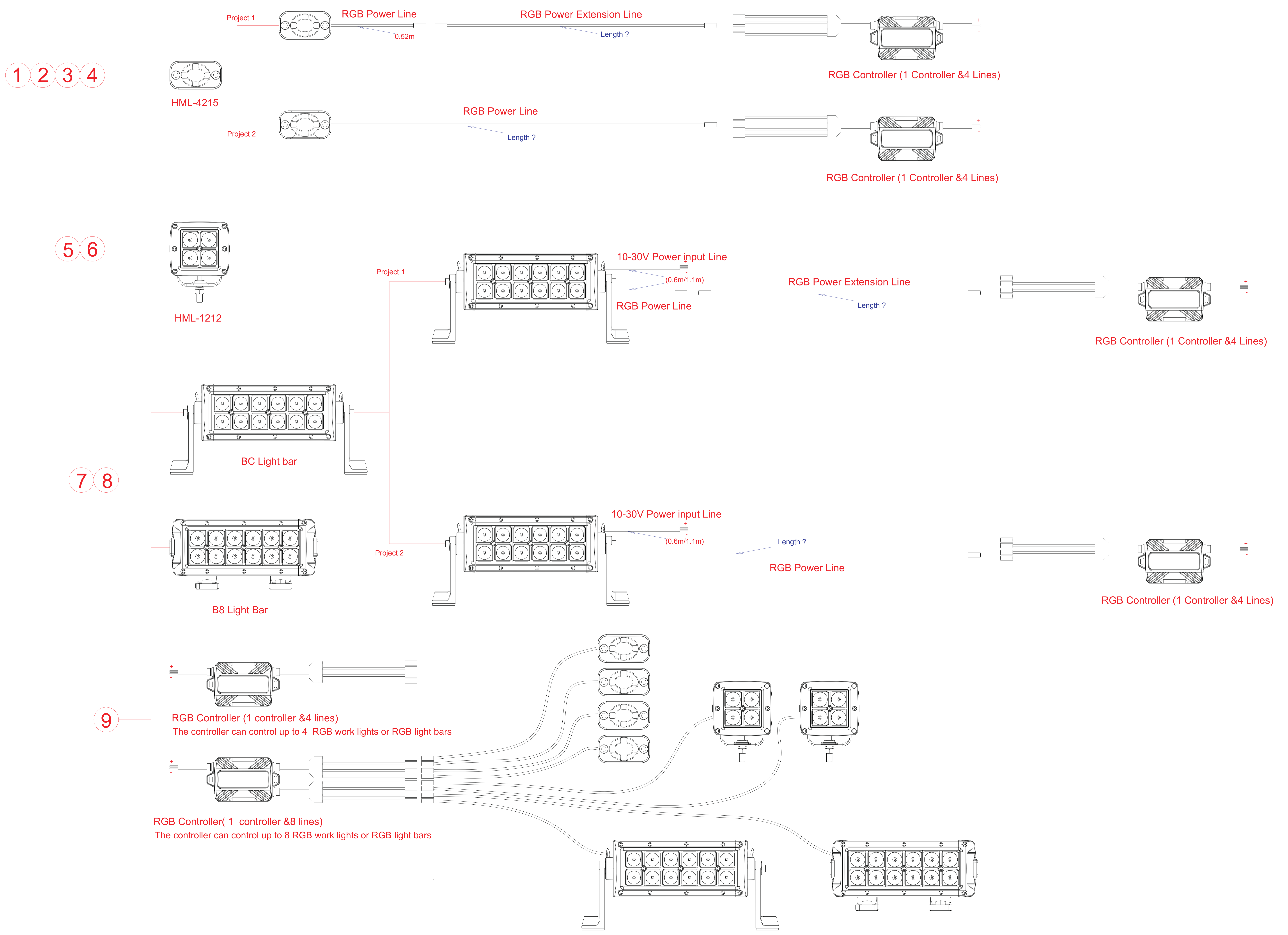
Lights Installation Drawing
